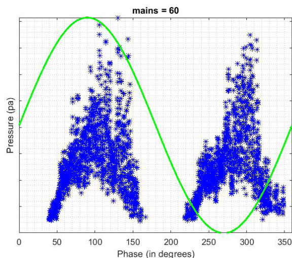
Figure 4: The PRDP analysis of an electrical discharge detected on a power transformer. The supply voltage frequency is 60 Hz and denoted with the green sinusoid.
